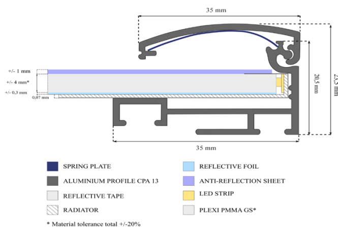
TECHNICAL CROSS SECTION CPA 13
